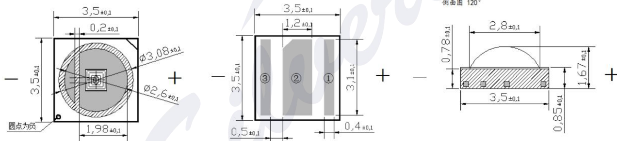
焊点结构 Pad Configuration:
